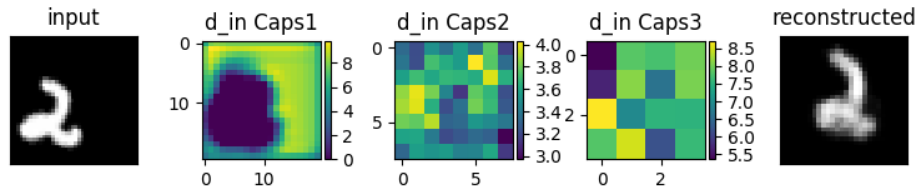
Figure 3: Visualization of dissimilarity maps and the reconstruction on affNIST. The heatmaps d_{in} are the inputs to the corresponding capsule layers.
