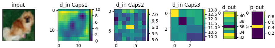
Figure 5: Visualization of dissimilarity maps on CIFAR-10. The heatmaps d\_in are the inputs to the corresponding capsule layers. p\_out is the transformation of d\_out to a probability vector containing probability values obtained by the negative softmax function.
