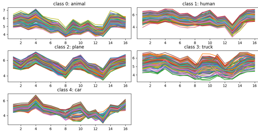
Figure 13: Line plot of the dissimilarity inputs of Caps3 over 100 digits per class of the smallNORB test dataset.
