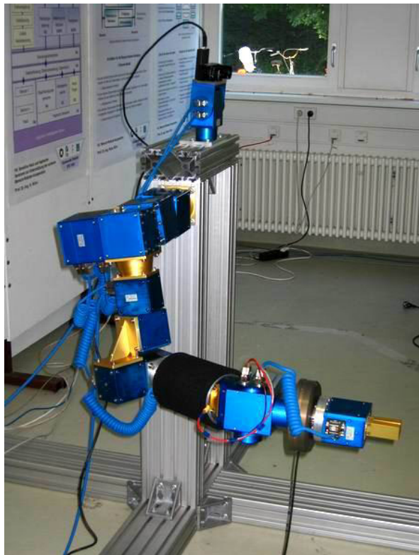
Fig. 5 Experimental setup
